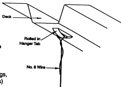
Integral Hanger Tab Allowable load 100 lb. (Types 20, 18, & 16) (Not to be used for suspended plaster ceilings, walkways, and/or utilities)
